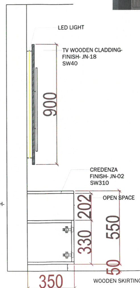
SKIRTING FINISH- JN-02 SW310 SIDE VIEW
