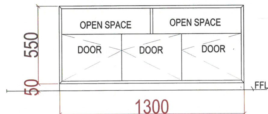
FRONT VIEW- CREDENZA WITH TV CLADDING-02
